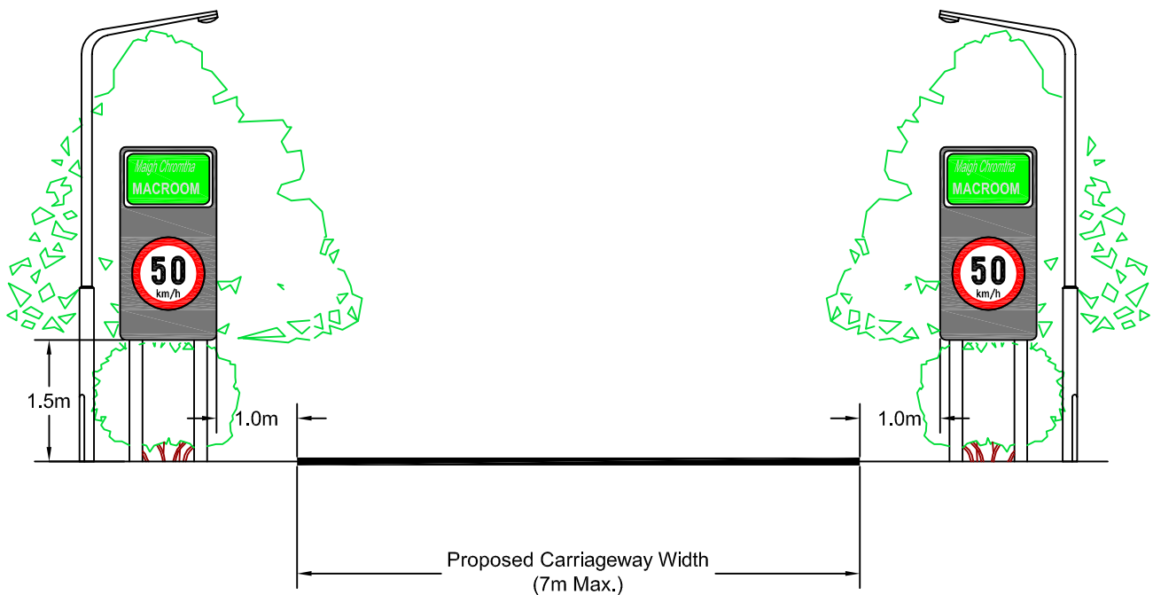
GATEWAY ELEVATION: TYPE 1 DESIGN PLATE No. 8
