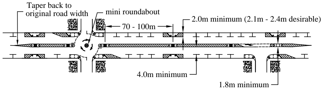
ROAD WIDTH > 13.8m PLATE No. 30
